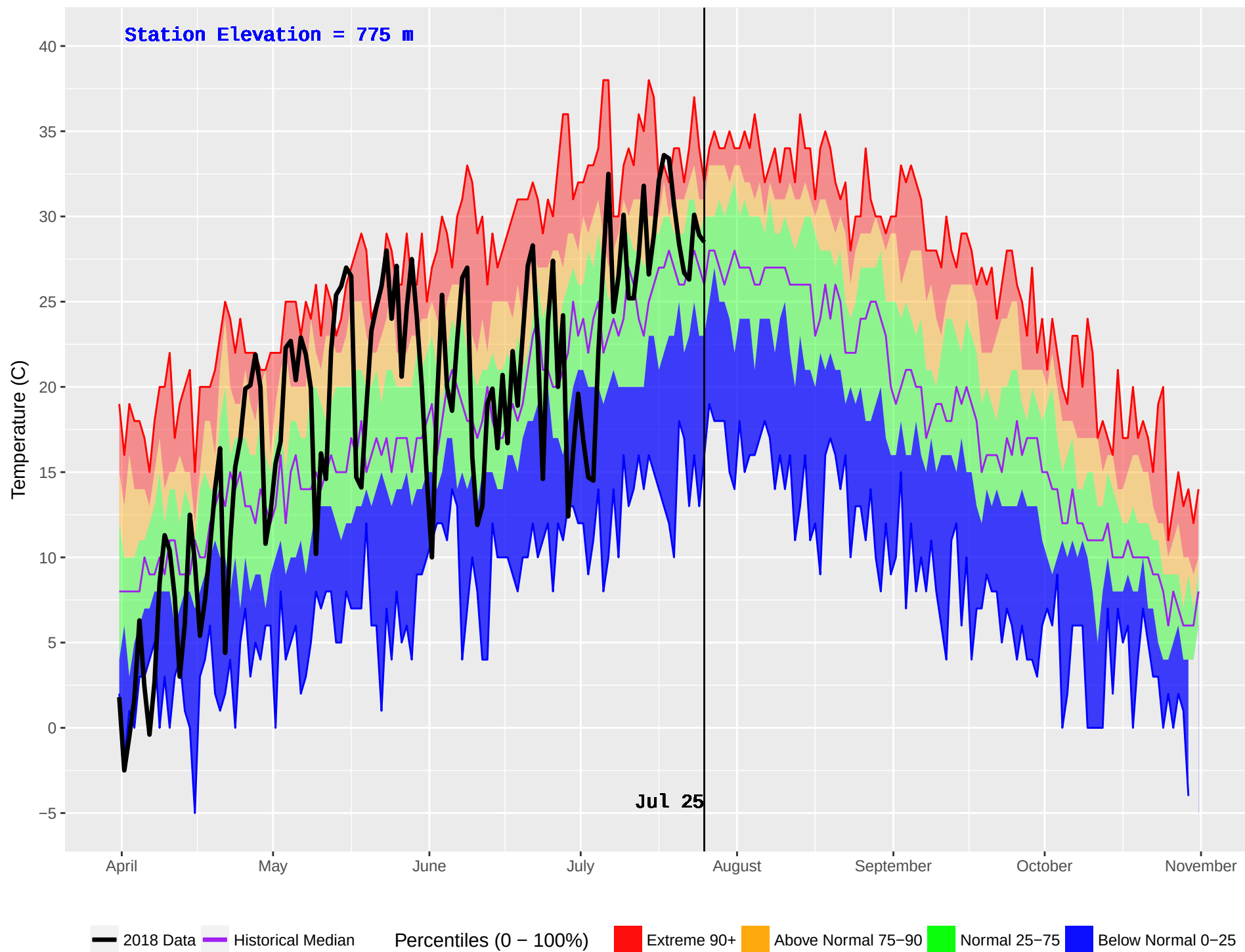
ELKO (412) : Historical (1970–2016) and Current (2018) Noon Temperature
